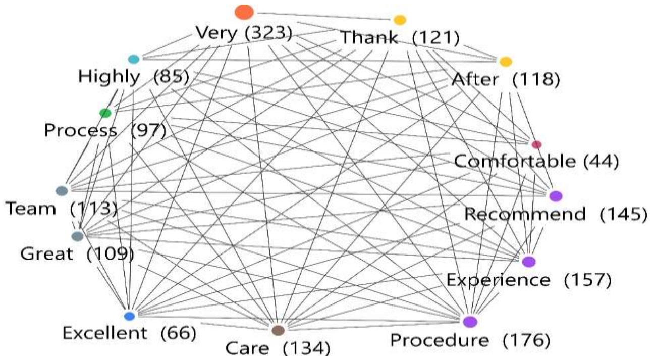
Figure 8. Code Map
